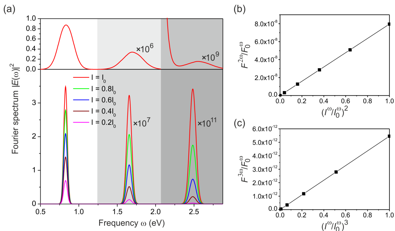
Figure 2. (a) Nonlinear scattering spectra from the infinitely long Au cylinder of 100 nm radius simulated for the excitation pulse of \tau = 5 fs (top) and \tau = 20 fs (bottom). (b, c) Integrated flux F^{2\omega} for (b) SHG and (c) THG normalized to the maximum incident fundamental flux F_0^\omega (corresponding to the peak intensity I_0^\omega ) as a function of the fundamental light intensity.
